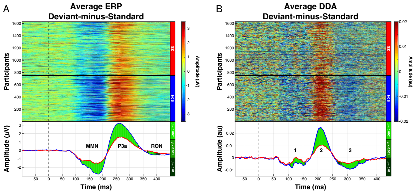
Fig. 1. DDA identified dynamical state changes preceding each of the ADR complex components. (A) NCSs demonstrated robust MMN, P3a, and RON components as shown in the heat map of the individual subject difference (deviant tone ERP – standard tone ERP) average signals ( Upper ). All three components of the ADR (MMN, P3a, and RON) can be appreciated in the group-level average signals ( Lower ). (B) DDA a_3 coefficient values averaged within each subject revealed significantly decreased a_3 in the SZ patients ( Upper ). As with the ERP results, the DDA group averages displayed three components with homologous waveform morphology and severity of deficits in SZ, but the DDA components (numbered 1–3 in Lower ) preceded their corresponding ERP peaks identified in A by 71, 54, and 82 ms, respectively. The shaded regions in the group average signals represent group differences that are statistically significant after adjusting for multiple comparisons (false discovery rate). Cohen's d , t values, and degrees of freedom are shown in SI Appendix, Fig. S9 .
