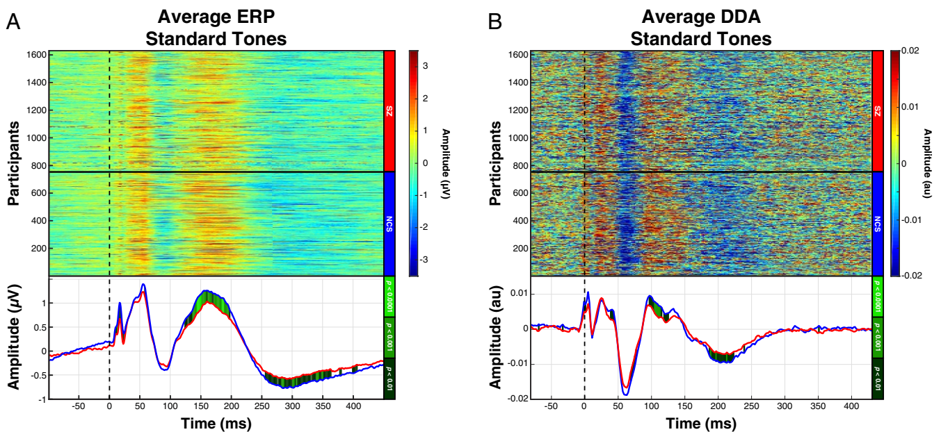
Fig. 3. DDA of standard tones detected significant dynamical state alterations preceding the P150 window. (A) ERP signals corresponding to the standard tones revealed a reduced P150 component in the SZ grand average signal (Lower). (B) Dynamic changes preceding the P150 ERP changes were observed in the 90- to 130-ms window (Lower; mean t value = 3.3, mean Cohen's d = 0.17). The a_3 changes were reduced for the SZ group during this time window.
