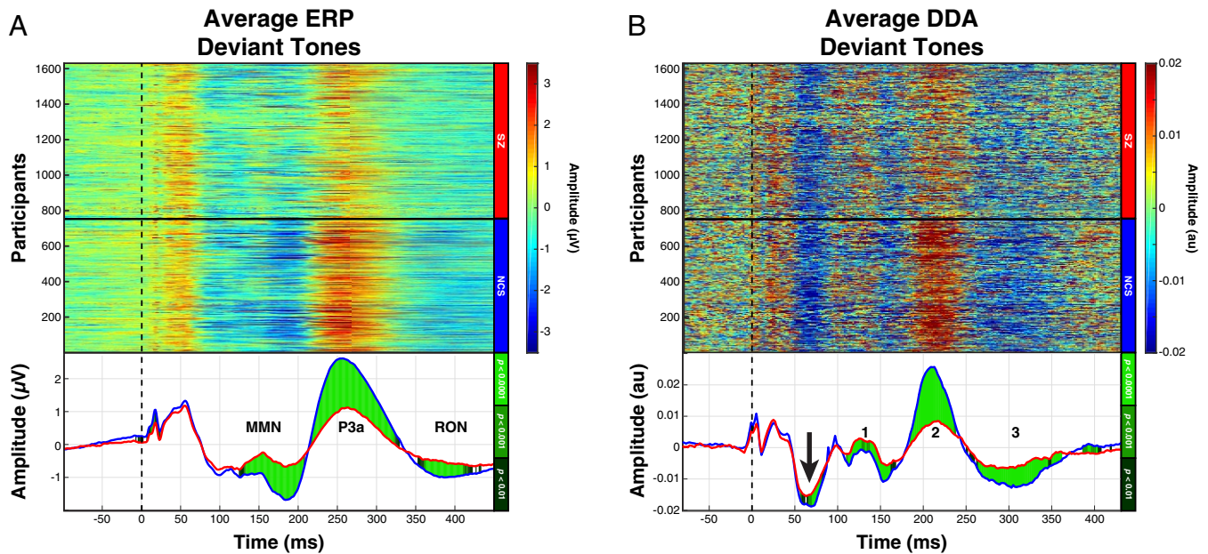
Fig. 2. ADR components were evident from both ERP analysis and DDA of waveforms elicited by deviant auditory tones. (A) Individual subject average signals from deviant tones revealed pronounced MMN and P3a components in the NCSs ( Upper ). The grand average signals from the two groups showed significantly different ADR component signals ( Lower ). (B) DDA a_3 amplitude changes were observed before each of the ADR components (numbered 1–3 in Lower ). Furthermore, statistically significant differences in a_3 amplitude between groups were detected during the earliest time window (50–100 which ms) in an auditory tone could be processed as deviant (black arrow; mean t value = -2.6 , mean Cohen's d = -0.13 ).
